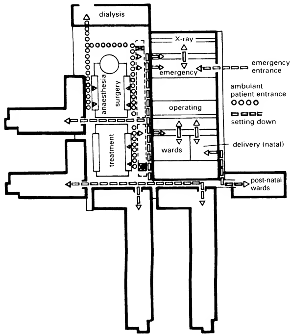
③ Internal connections, Prignitz Hospital Architects: B + C Lambart
